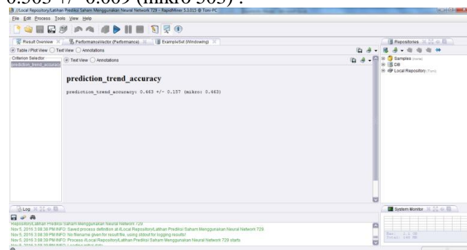
Gambar 4.1.1. Performance Prediction Trend Accuracy 729 Dataset Menggunakan Neural Network
