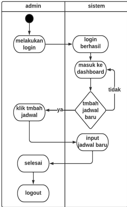
Gambar 5. Activity Diagram Admin
