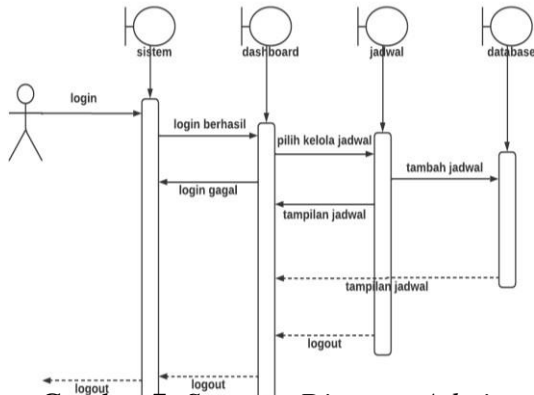
Gambar 7. Squence Diagram Admin
