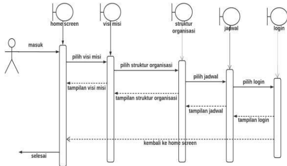
Gambar 8. Squence Diagram User
