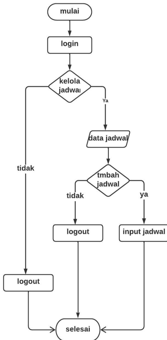
Gambar 1. Flowchart Admin
