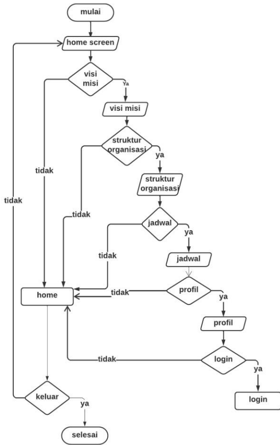
Gambar 2. Flowchart User
