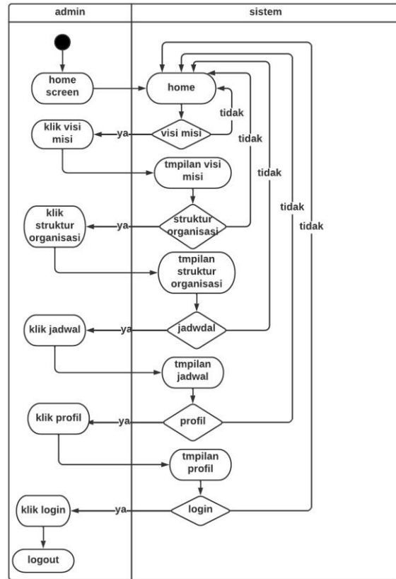
Gambar 6. Activity Diagram User
