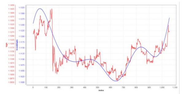
Gambar 11 Kernel Radial
