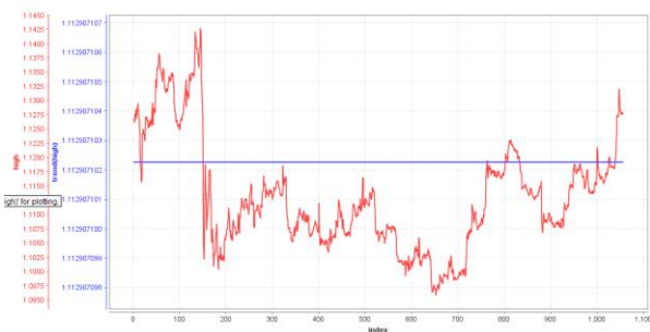
Gambar 8 Kernel Multiquaric
