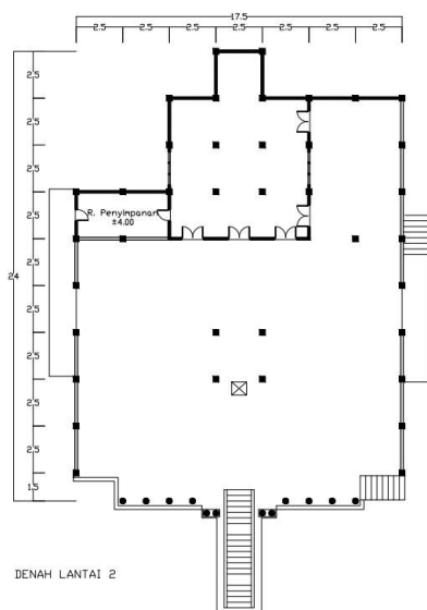
Gambar 3 Denah Lantai 2 Masjid Jami' Sunan Abinawa
