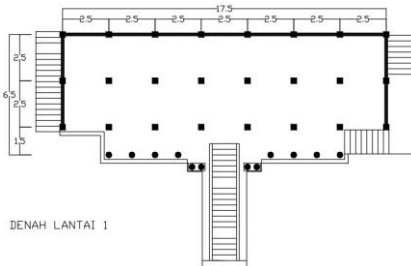
Gambar 2 Denah Lantai 1 Masjid Jami' Sunan Abinawa
